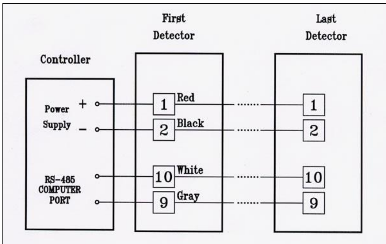
Figure 10: RS-485 Networking
