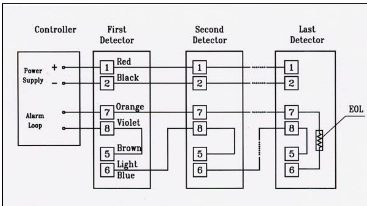
Figure 13: Typical Wiring for 4 Wire Controllers
